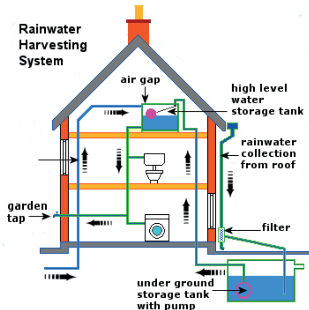
Rainwater harvesting (Source: Taylors of Bath)
